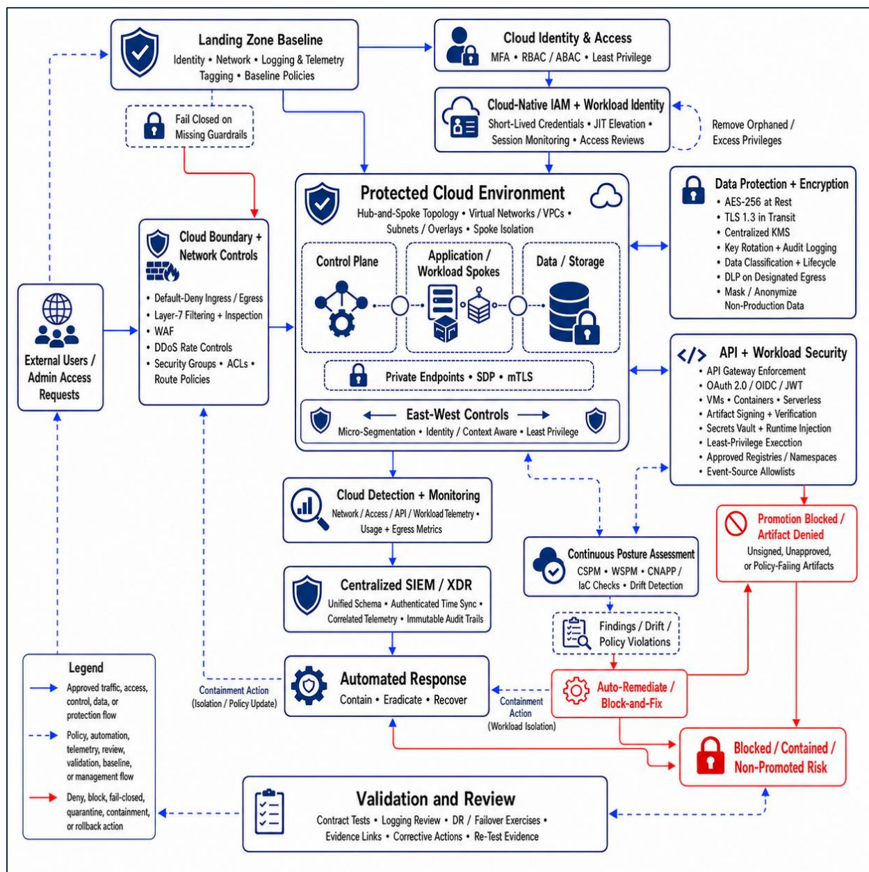
Figure 6-1. This illustrates the Defensible Cloud Security Architecture output model for Section 6. The model shows how landing zone baselines, cloud identity and access controls, cloud boundary protections, hub-and-spoke segmentation, data protection, API and workload security, monitoring, automated response, posture assessment, and validation activities work together to establish measurable, enforceable, and auditable cloud security outcomes.
