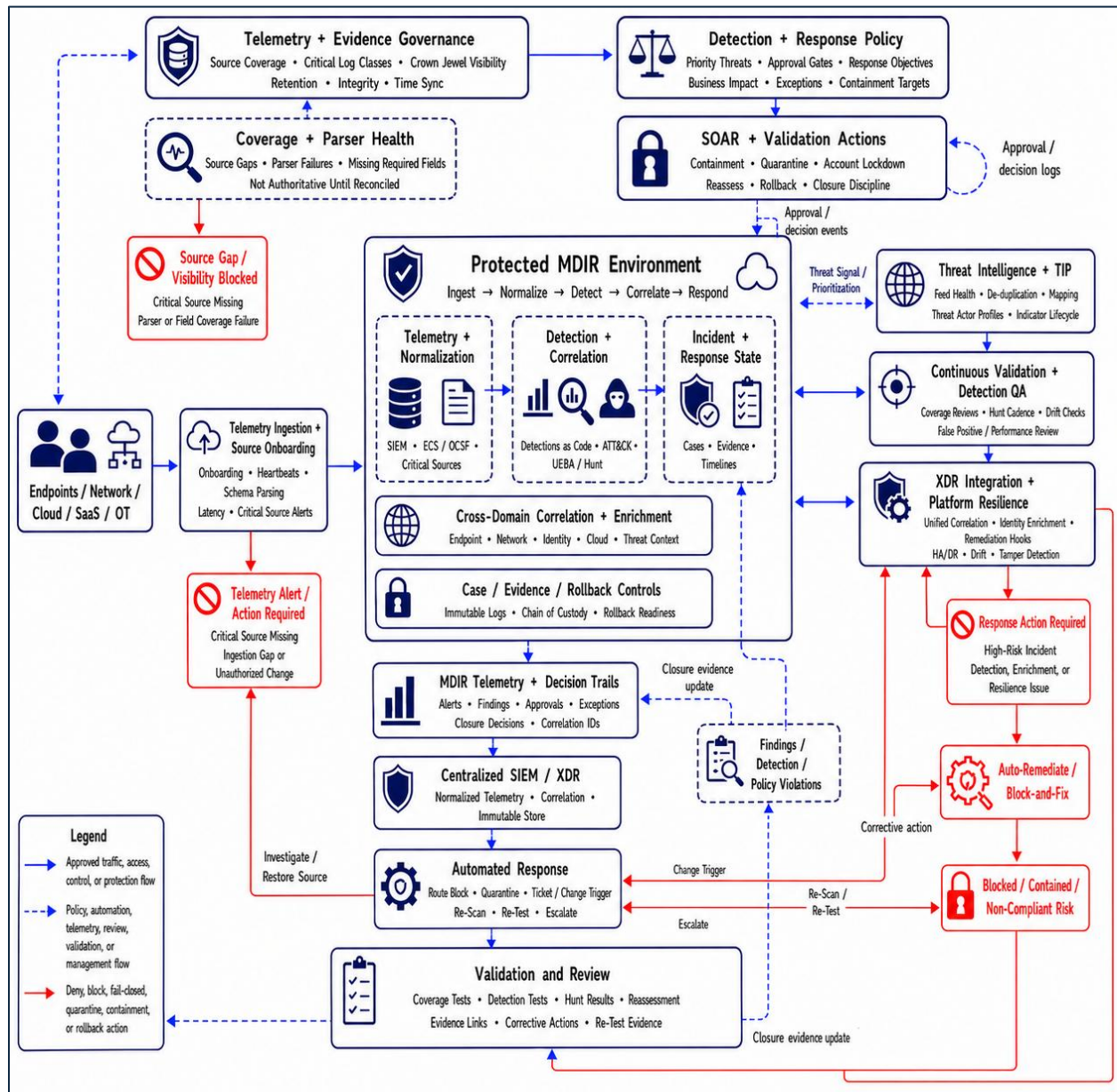
Figure 6-1. This illustrates the Defensible Monitoring, Detection, and Incident Response output model for Section 6. The model shows how telemetry governance, source onboarding, parser health, detection engineering, threat intelligence, SOAR validation, XDR integration, incident response state, evidence handling, automated response, continuous validation, and review activities work together to establish measurable, enforceable, auditable monitoring, detection, and response outcomes.
